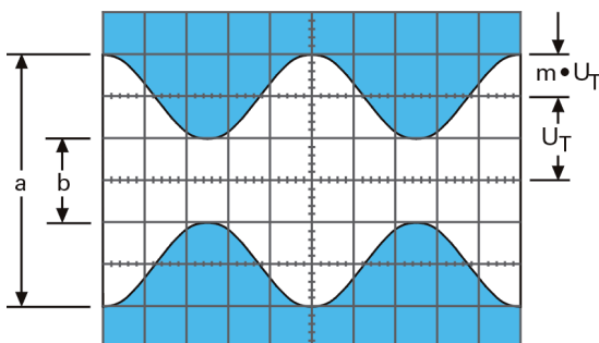
Picture 2: Amplitude modulated hf. F = 1 \text{ MHz} , f = 1 \text{ kHz} ,
